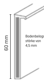
D 60 (without sealing lip)
